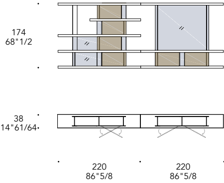
Example 2_ 440 x 38 x 174 h Tango T box
